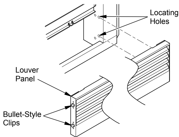
Removing Louver Panel with Bullet-Style Clips Figure: 4 (Direct-Vent Models)
