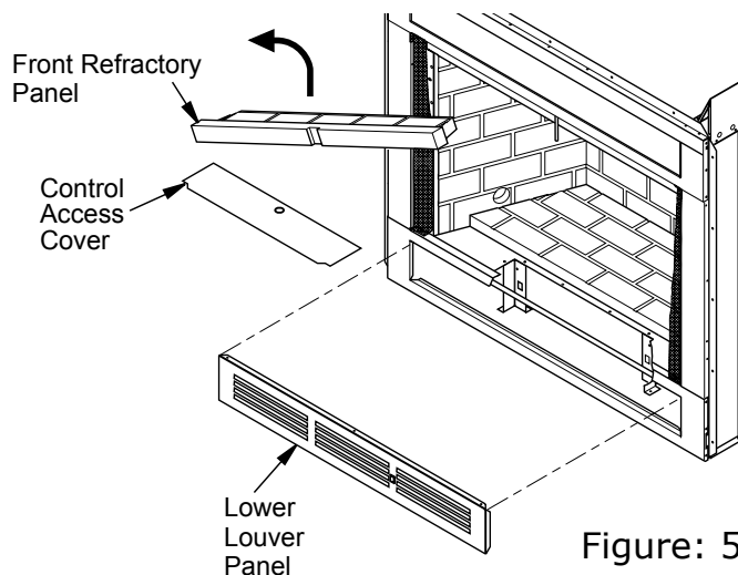
Accessing Blower Compartment B-Vent, Wood and Vent-Free Models
