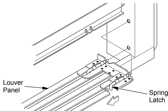
Removing Louver Panel with Spring Latches Figure: 3 (Direct-Vent Models)
